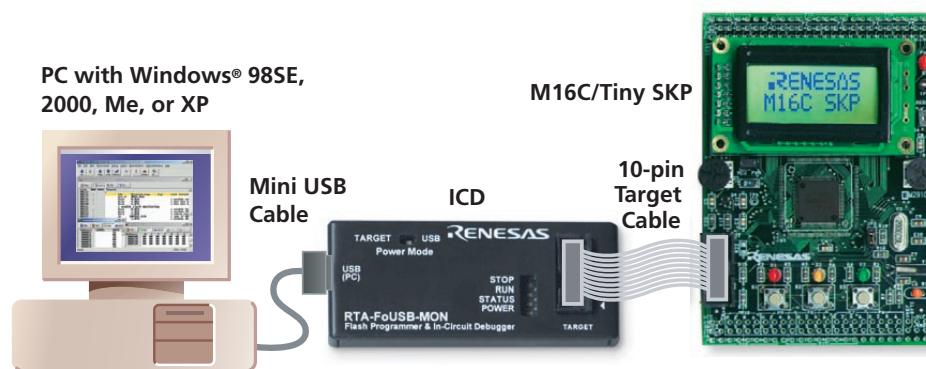
Figure 2. M16C/Tiny SKP System Connectivity
