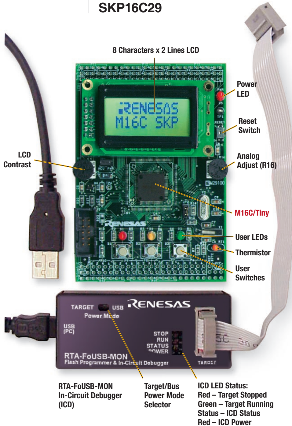
Figure 1. M16C/Tiny SKP
