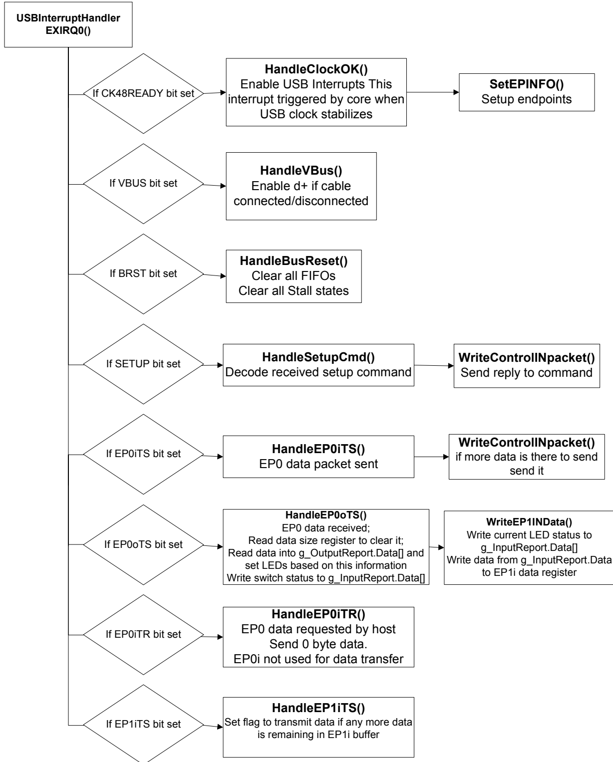
Figure 4: USBInterruptHandler EXIRQ0
