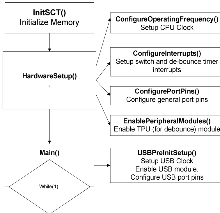
Figure 2: System Initialization
