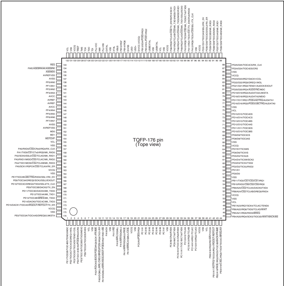
Figure 1.2 Pin Assignment
