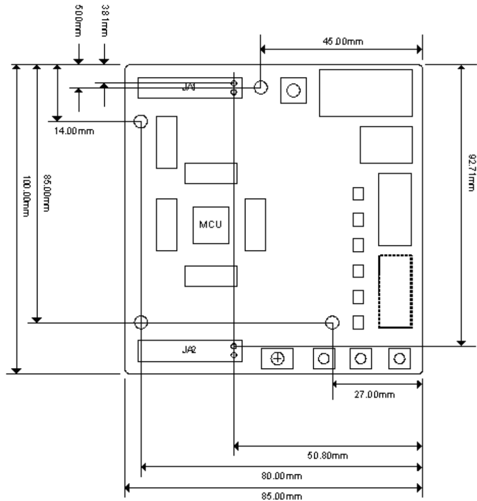
Figure C.1: RSK23 Board Dimensions
