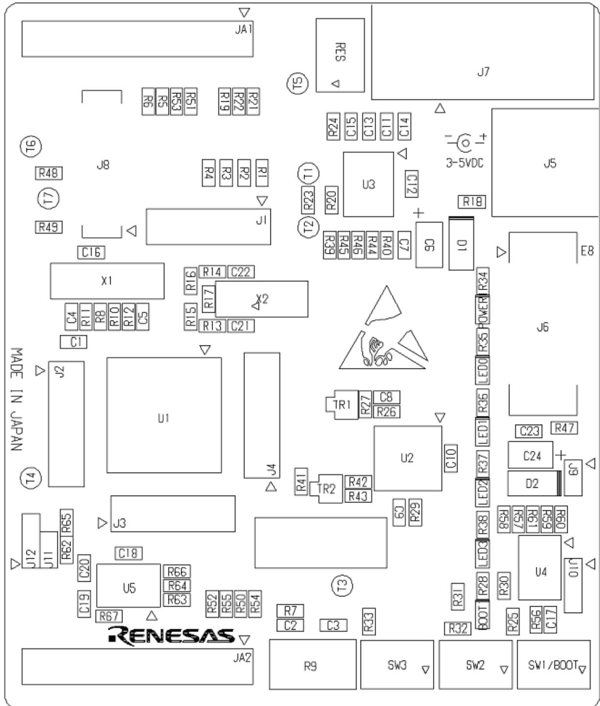
Figure B.1: RSK23 Component Layout
